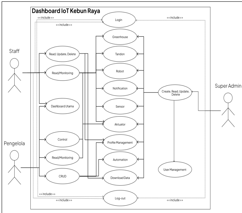
Gambar 3.3 Use Case Diagram Website ITERAHERO
