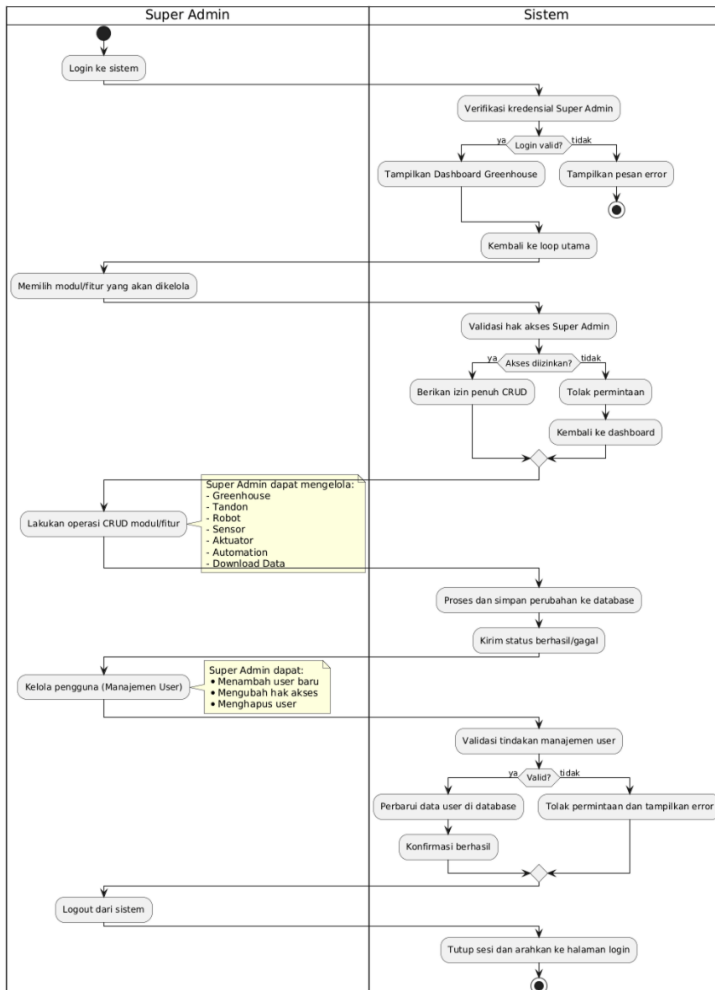
Gambar 3.6 Activity Diagram Super Admin
