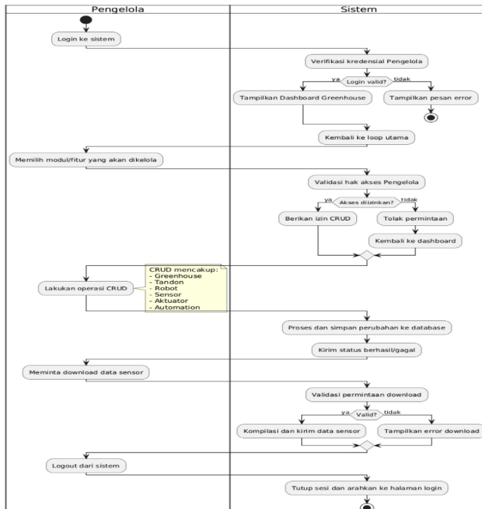
Gambar 3.5 Activity Diagram Pengelola
