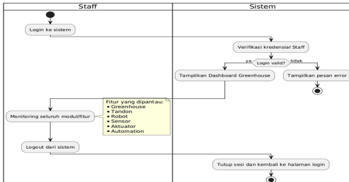
Gambar 3.4 Activity Diagram Staff
