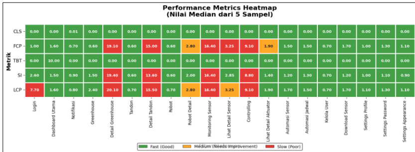
Gambar 3.2 Benchmark Performance Lighthouse Website
