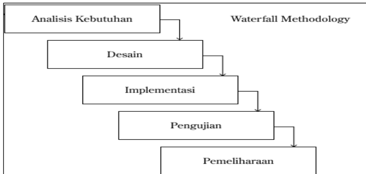
Gambar 2.2 Metode Waterfall
